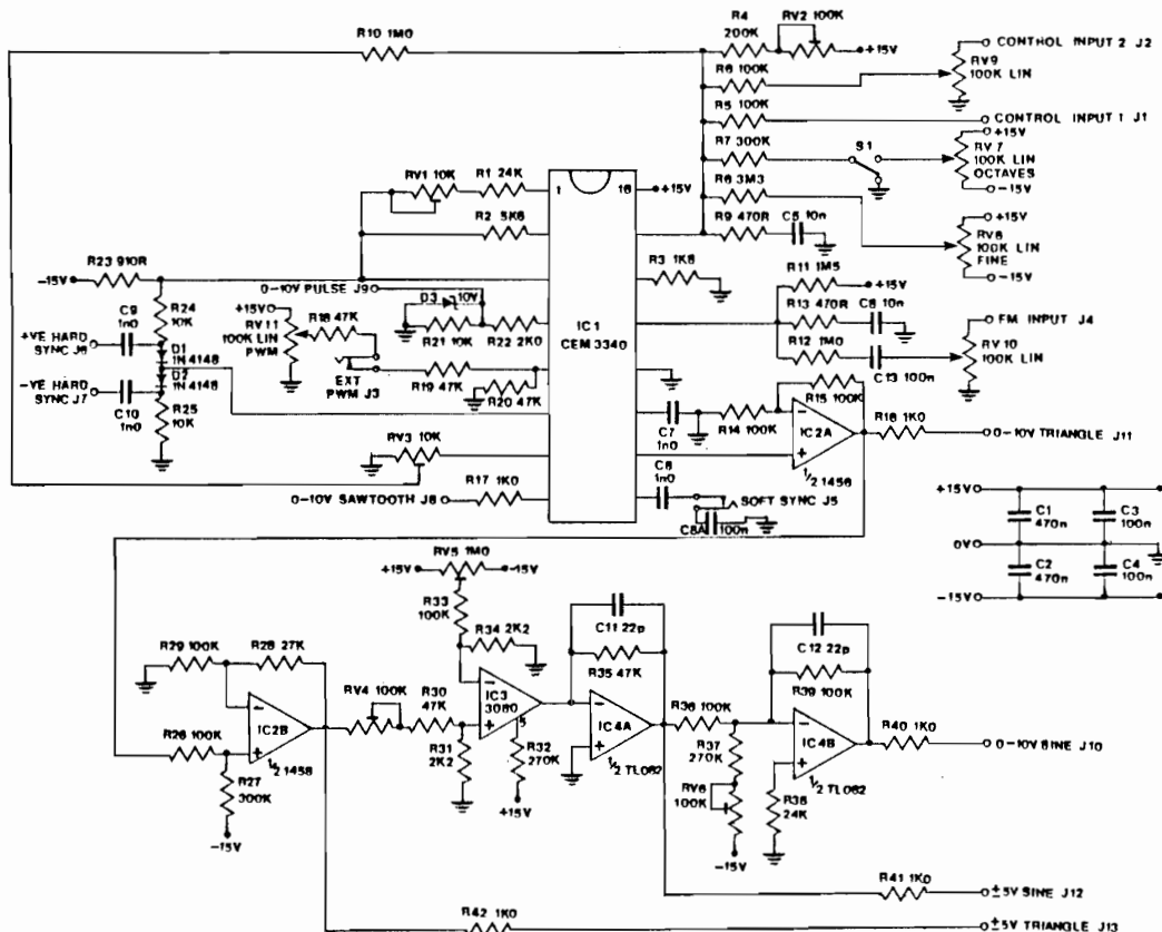
FIGURE 2. CIRCUIT FOR 80-2 VCO
