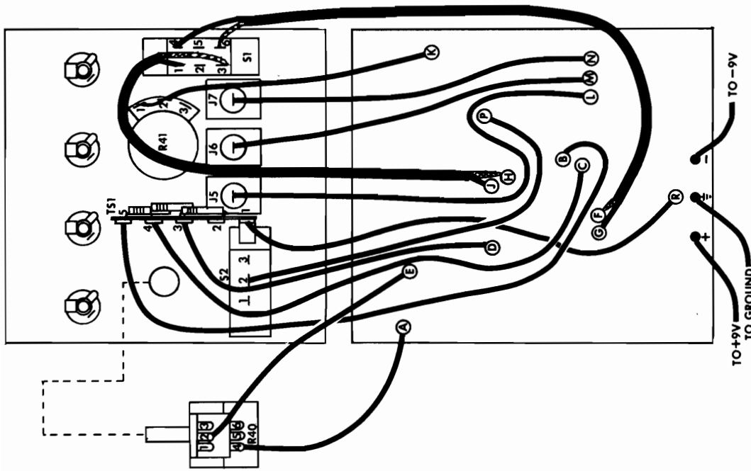
Figure 9 - Circuit board to front panel wiring detail. Previous wiring has been omitted for clarity.
