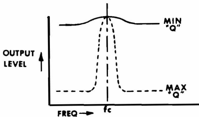
Figure 12 - Effect of varying Q on Band-Pass output.
