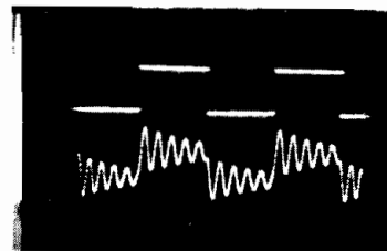
1 kHz. square wave input, LP VCF output Fc 5 kHz.
