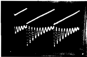
1 kHz. ramp input, LP VCF output Fc 10kHz.
